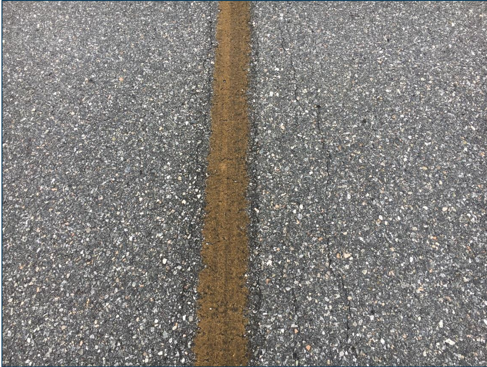
Taxiway A, Section 110, Sample Unit 141 – Low Severity (48) Longitudinal and Transverse Cracking, Low Severity (52) Raveling, Low Severity (57) Weathering
