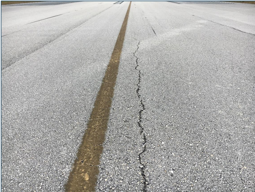
Runway 10-28, Section 6205, Sample Unit 157 – Low Severity (48) Longitudinal and Transverse Cracking, Low Severity (57) Weathering
