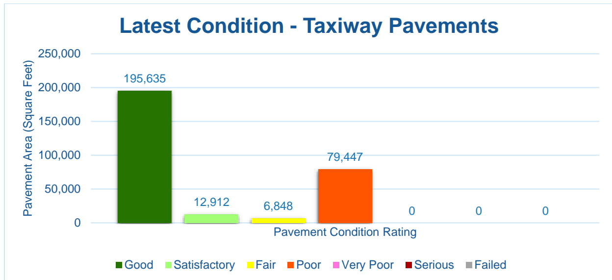
Figure 4.1.2 (b) Latest Condition – Taxiway Pavements
