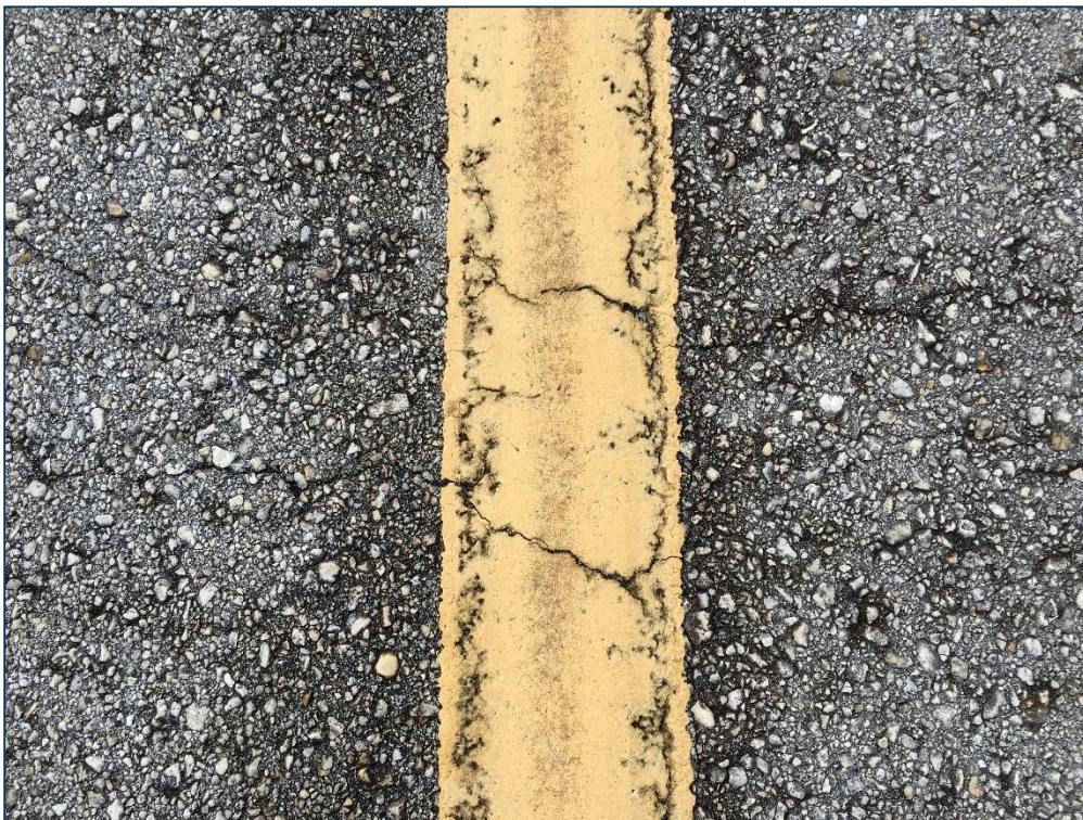
Taxiway A, Section 105, Sample Unit 131 – Low Severity (48) Longitudinal and Transverse Cracking, Low Severity (57) Weathering
