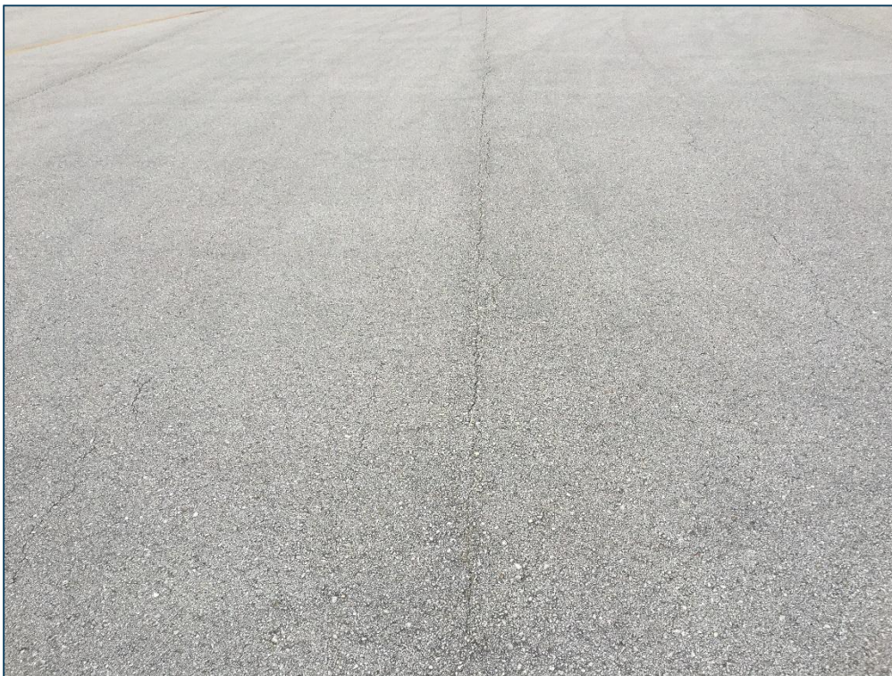
Taxiway A1, Section 305, Sample Unit 101 – Low Severity (48) Longitudinal and Transverse Cracking, Low Severity (57) Weathering
