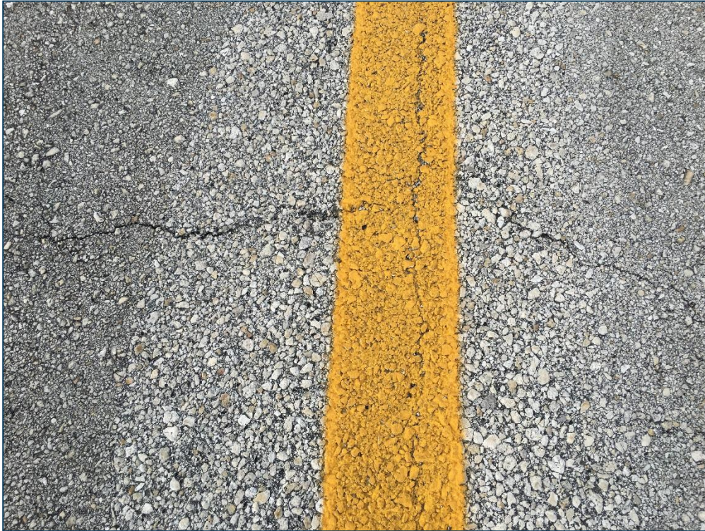
Taxiway A4, Section 605, Sample Unit 600 – Low Severity (48) Longitudinal and Transverse Cracking, Low Severity (57) Weathering
