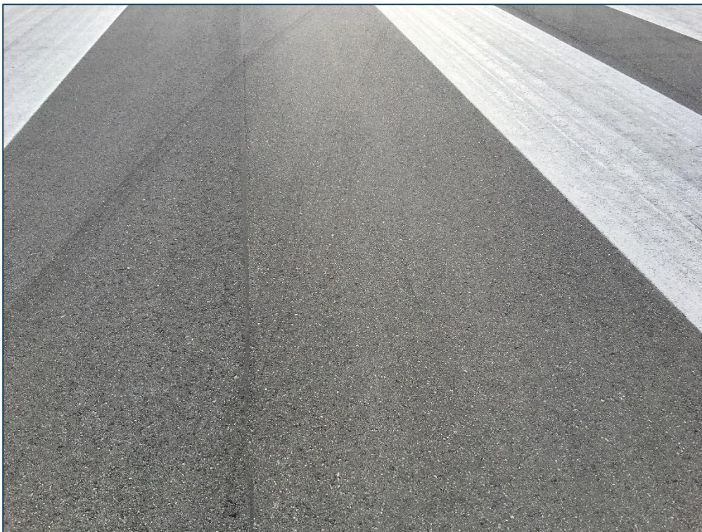
Runway 9-27, Section 6235, Sample Unit 397 – Low Severity (57) Weathering
