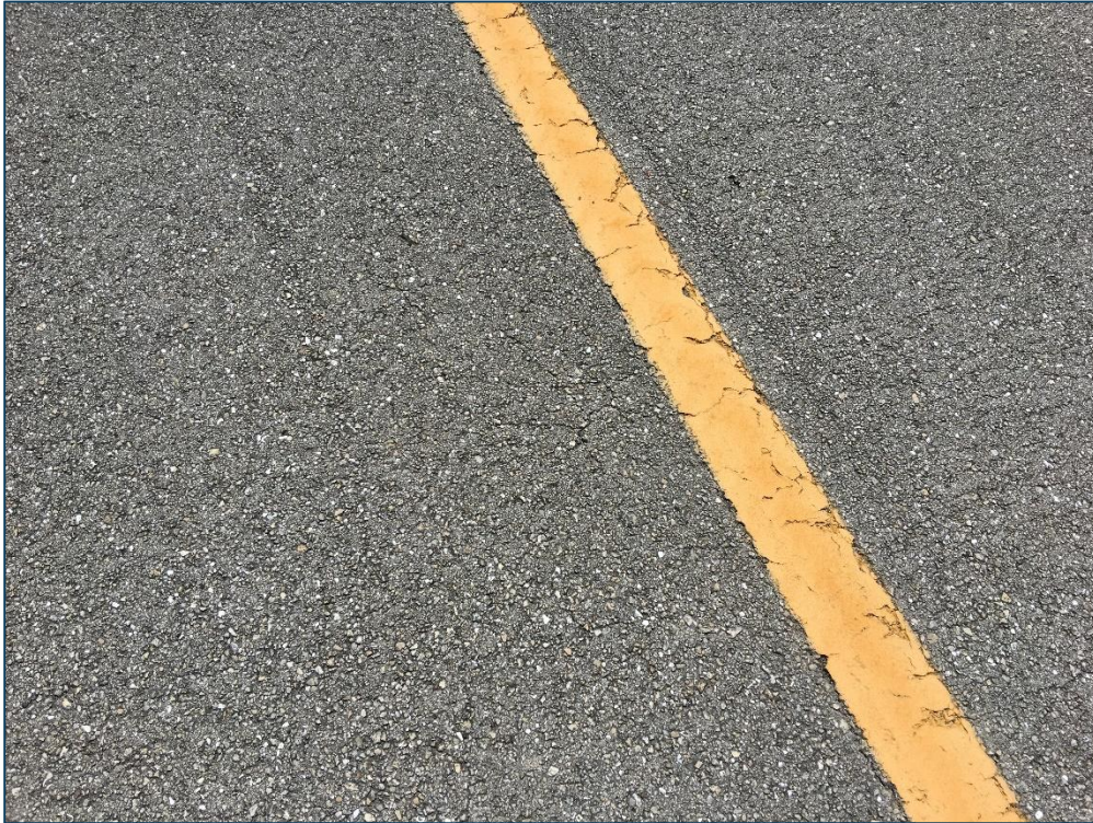
Taxiway A, Section 110, Sample Unit 204 – Low Severity (48) Longitudinal and Transverse Cracking, Low Severity (52) Raveling, Medium Severity (52) Raveling
