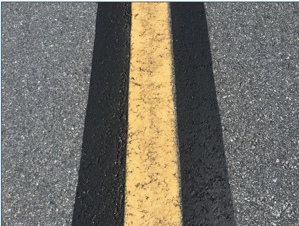
Taxiway A, Section 305, Sample Unit 116 – Low Severity (48) Longitudinal and Transverse Cracking, Low Severity (57) Weathering
