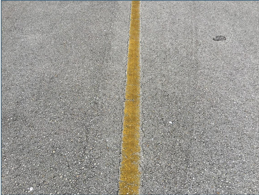
Apron AP, Section 4115, Sample Unit 100 – Low Severity (48) Longitudinal and Transverse Cracking, Medium Severity (52) Raveling, Low Severity (52) Raveling
