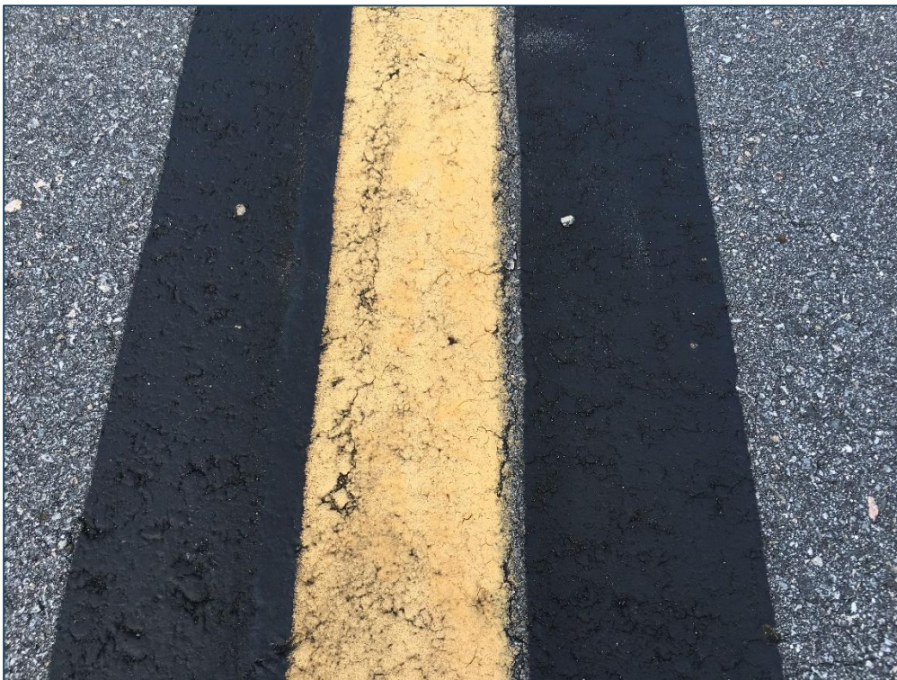
Taxiway A, Section 310, Sample Unit 200 – Low Severity (48) Longitudinal and Transverse Cracking, Low Severity (57) Weathering
