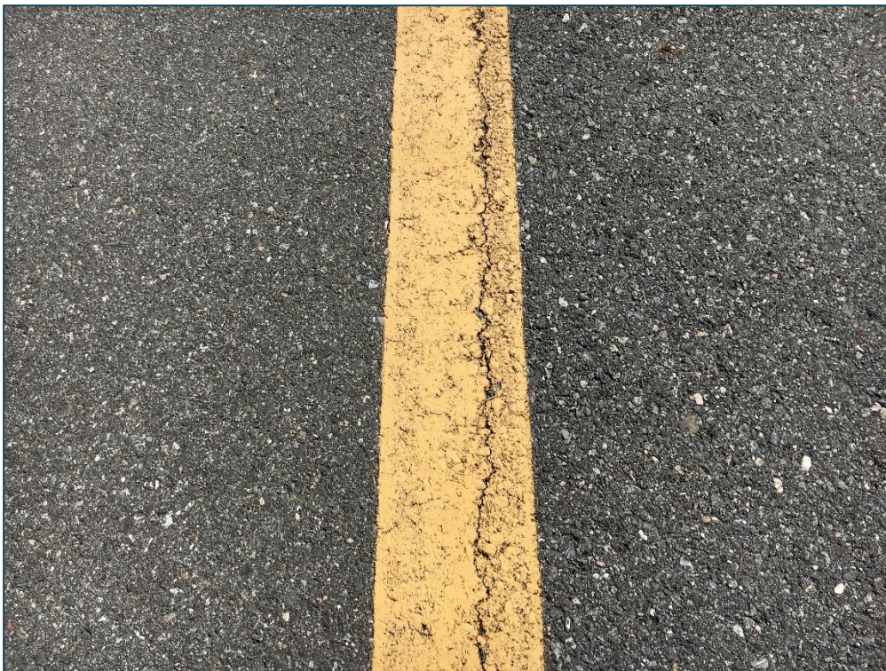
T-Hangar Taxilane, Section 4130, Sample Unit 101 – Low Severity (48) Longitudinal and Transverse Cracking, Low Severity (57) Weathering
