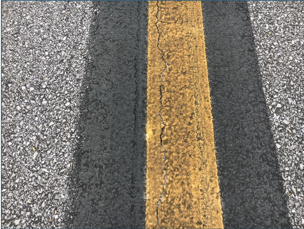
Taxiway A, Section 110, Sample Unit 101 – Low Severity (48) Longitudinal and Transverse Cracking, Low Severity (57) Weathering
