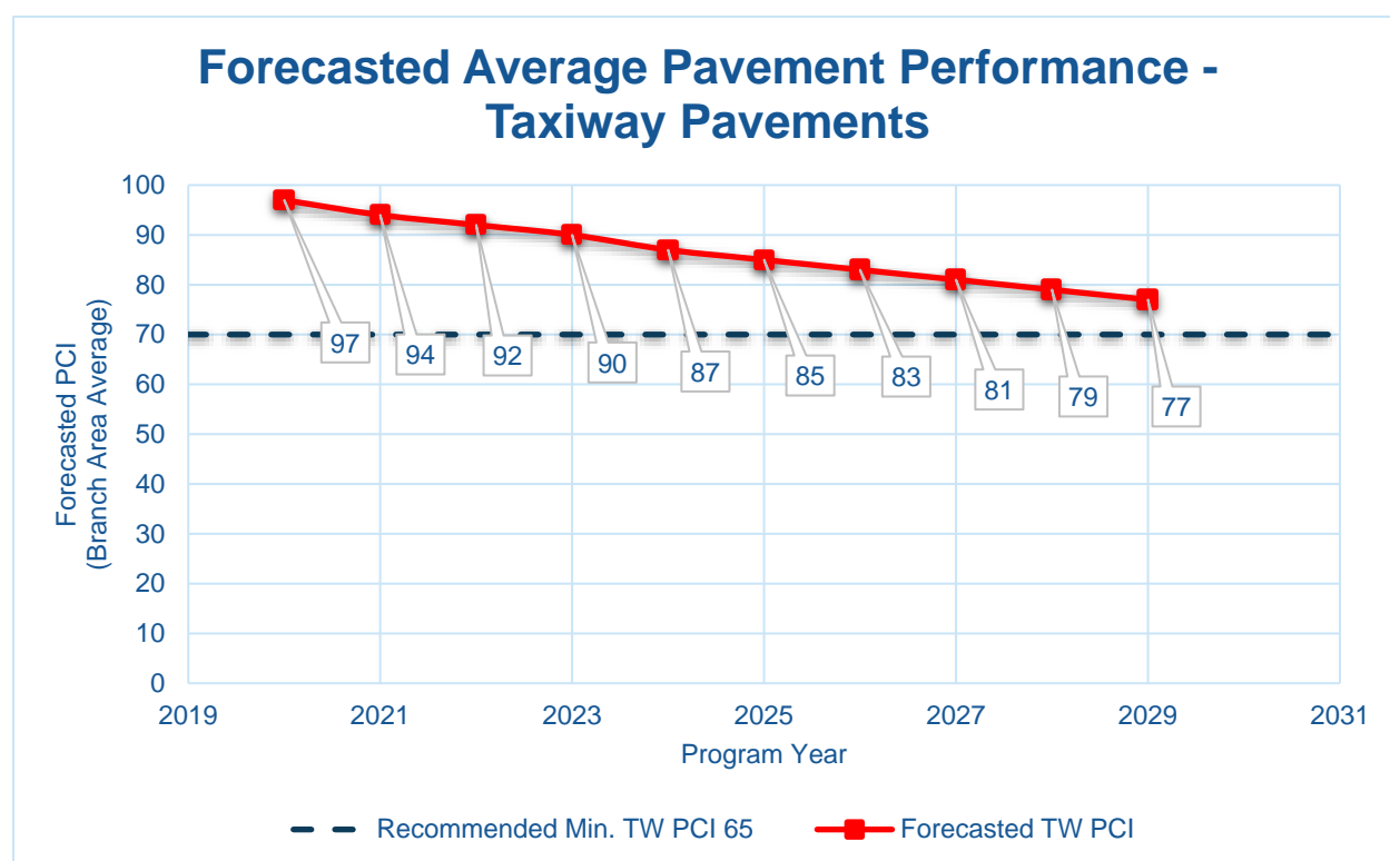
Figure 4.3.2 (a) Forecasted Taxiway Pavement Performance
