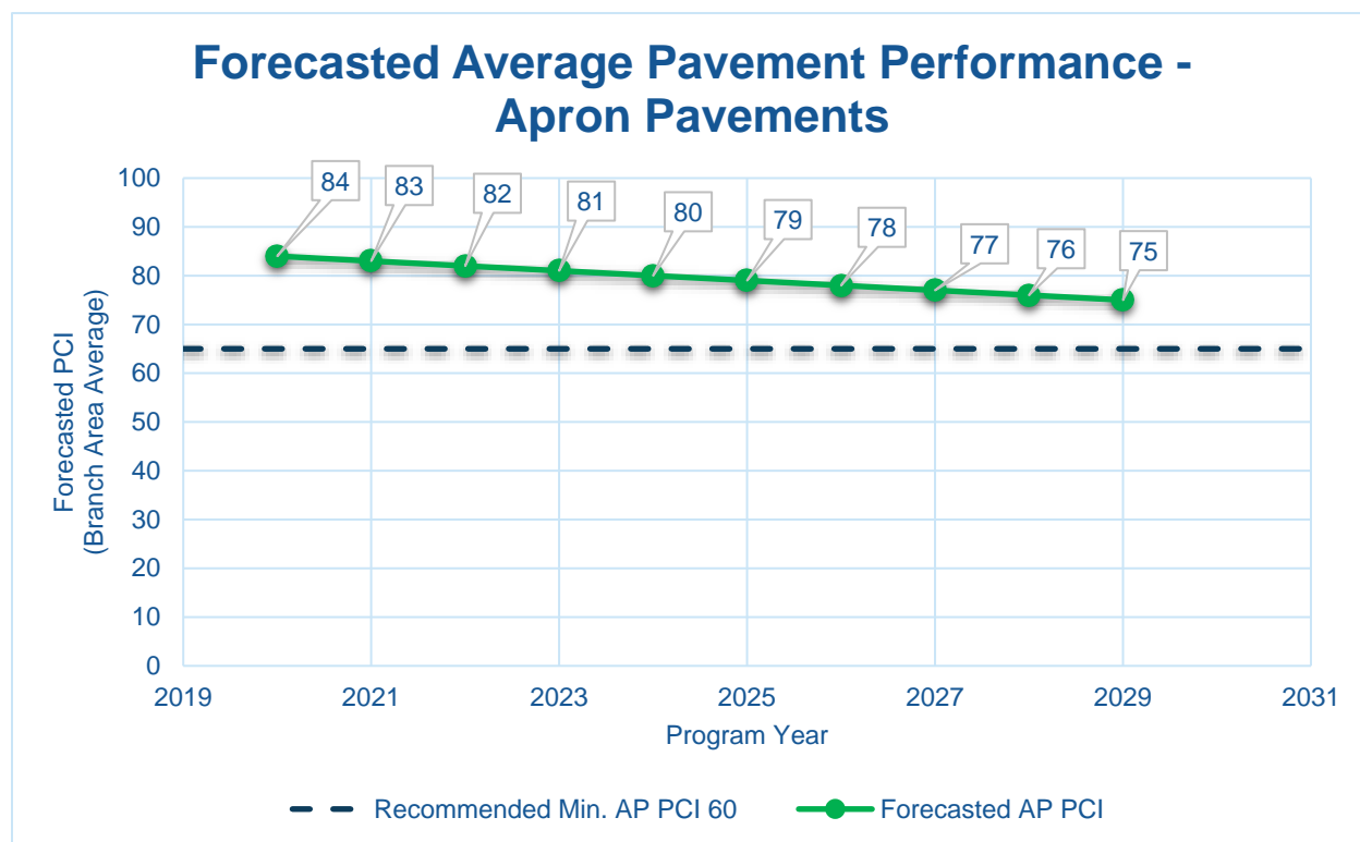
Figure 4.3.2 (b) Forecasted Apron Pavement Performance
