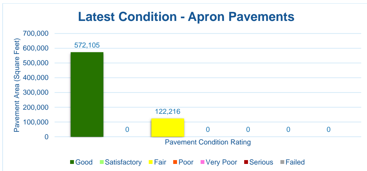
Figure 4.1.2 (b) Latest Condition – Apron Pavements
