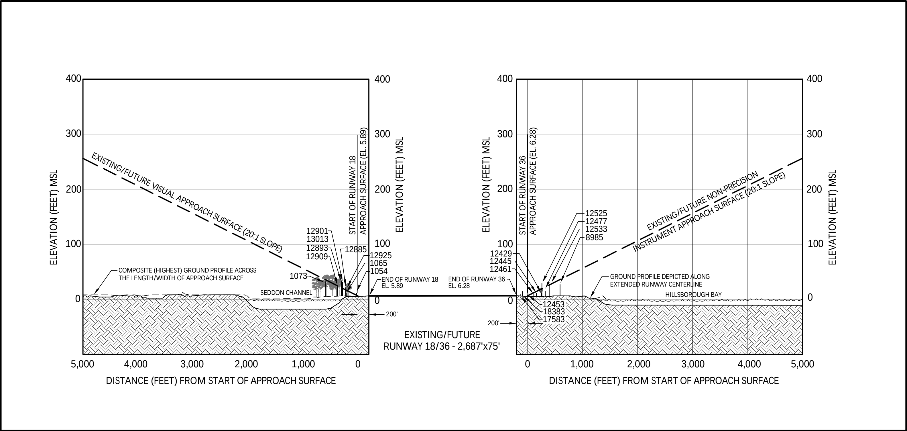
RUNWAY 18/36 PROFILE VIEW
