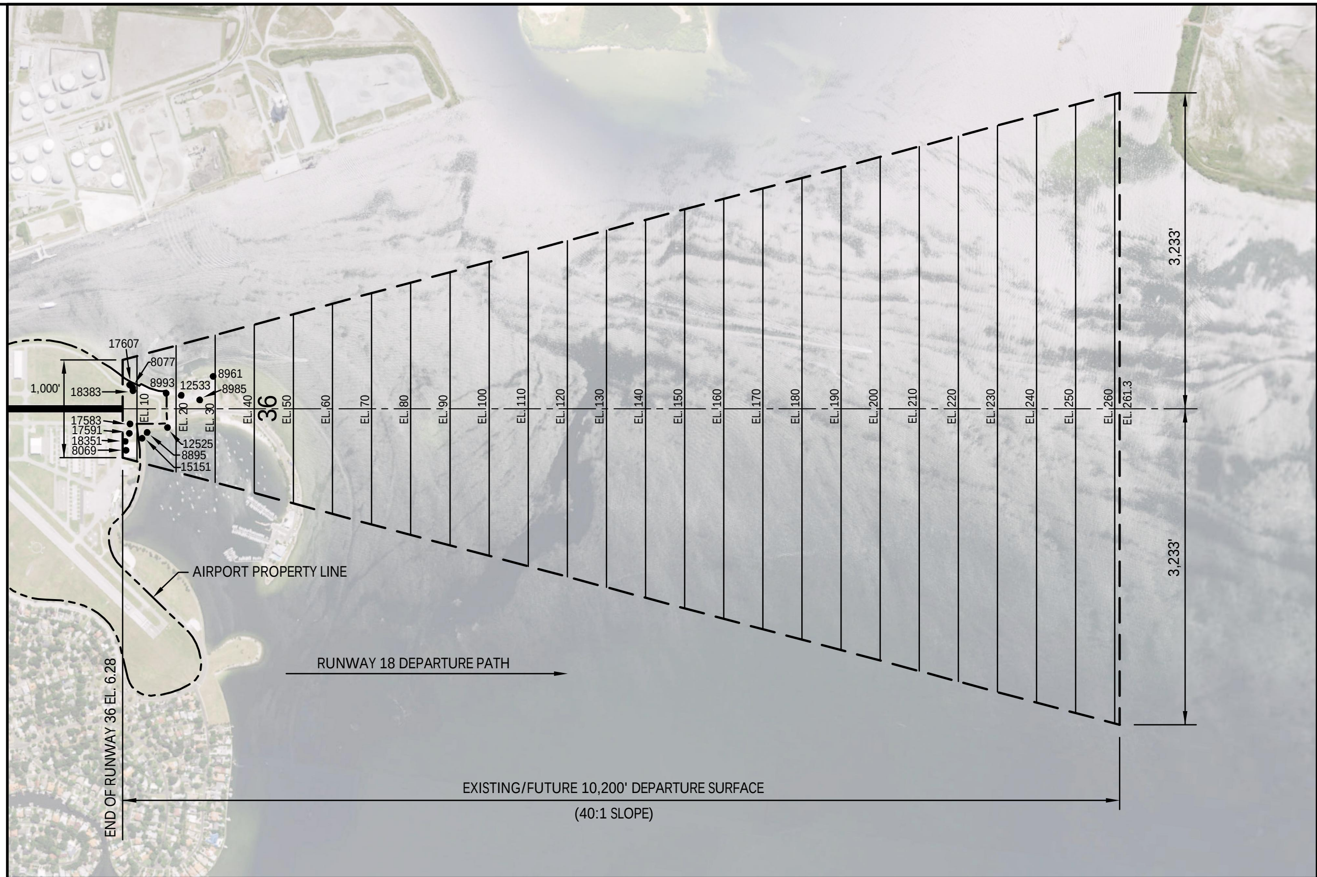
RUNWAY 18 DEPARTURE SURFACE PLAN VIEW
