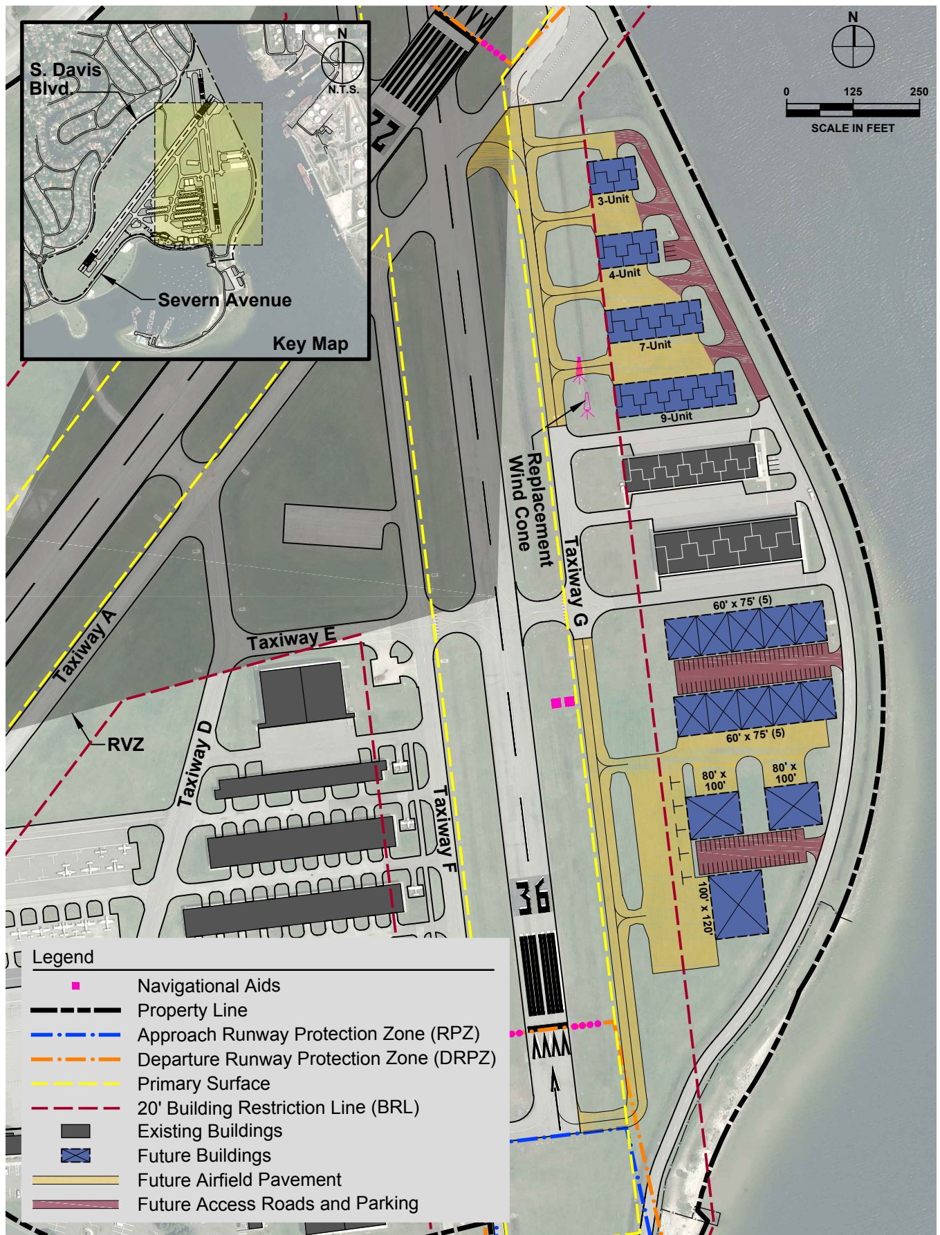
Figure 5-3 Landside Development Alternative 1
