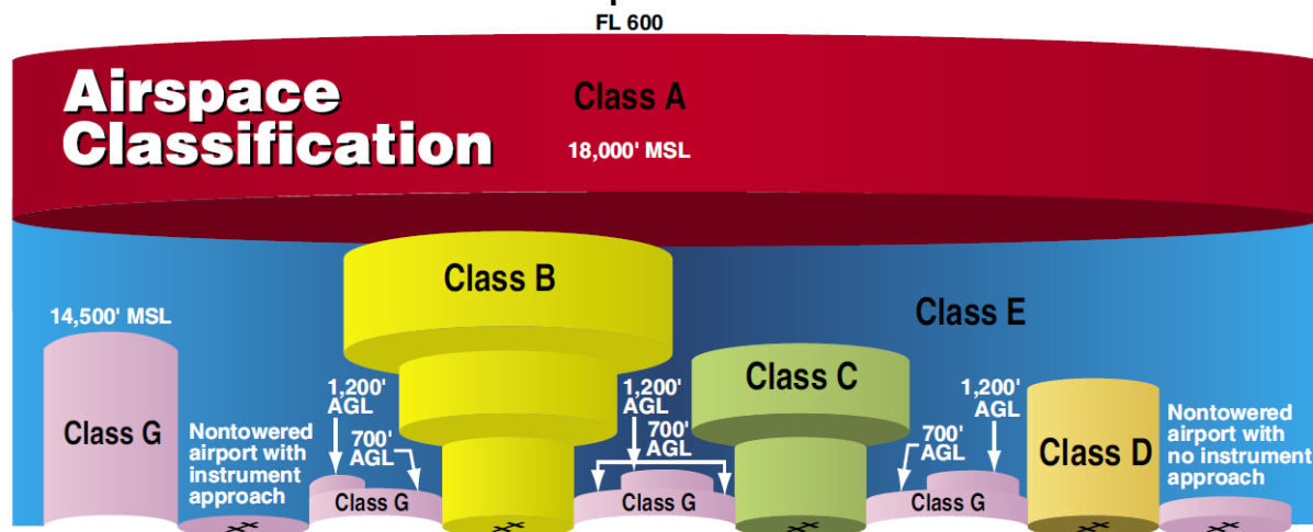
Figure 2-2 Airspace Classes
