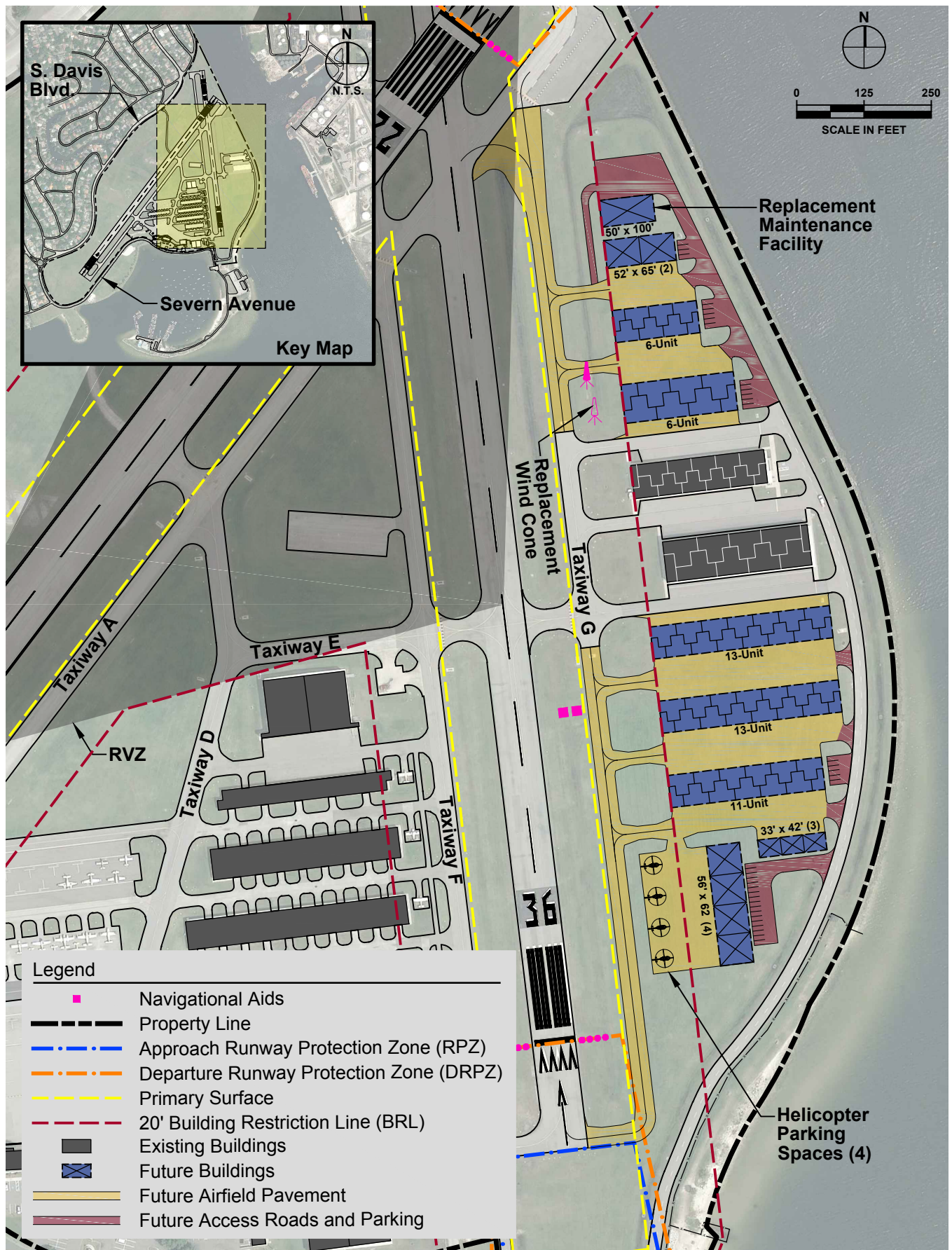
Figure 5-4 Landside Development Alternative 2
