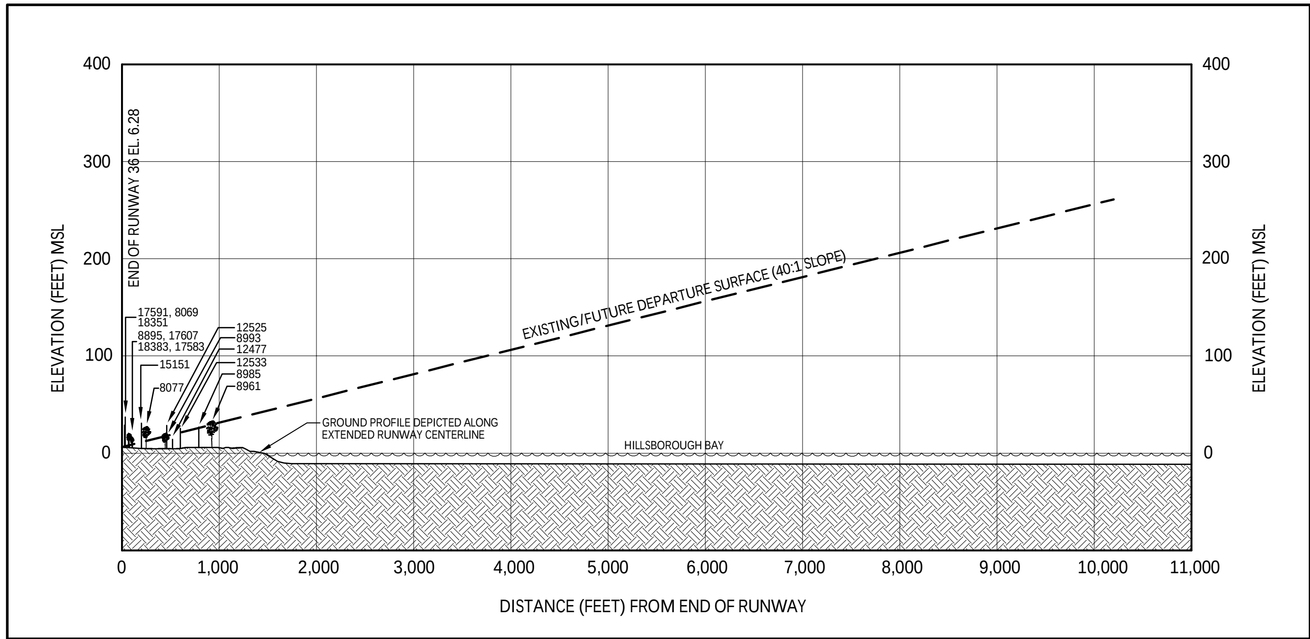
RUNWAY 18 DEPARTURE SURFACE PROFILE VIEW
