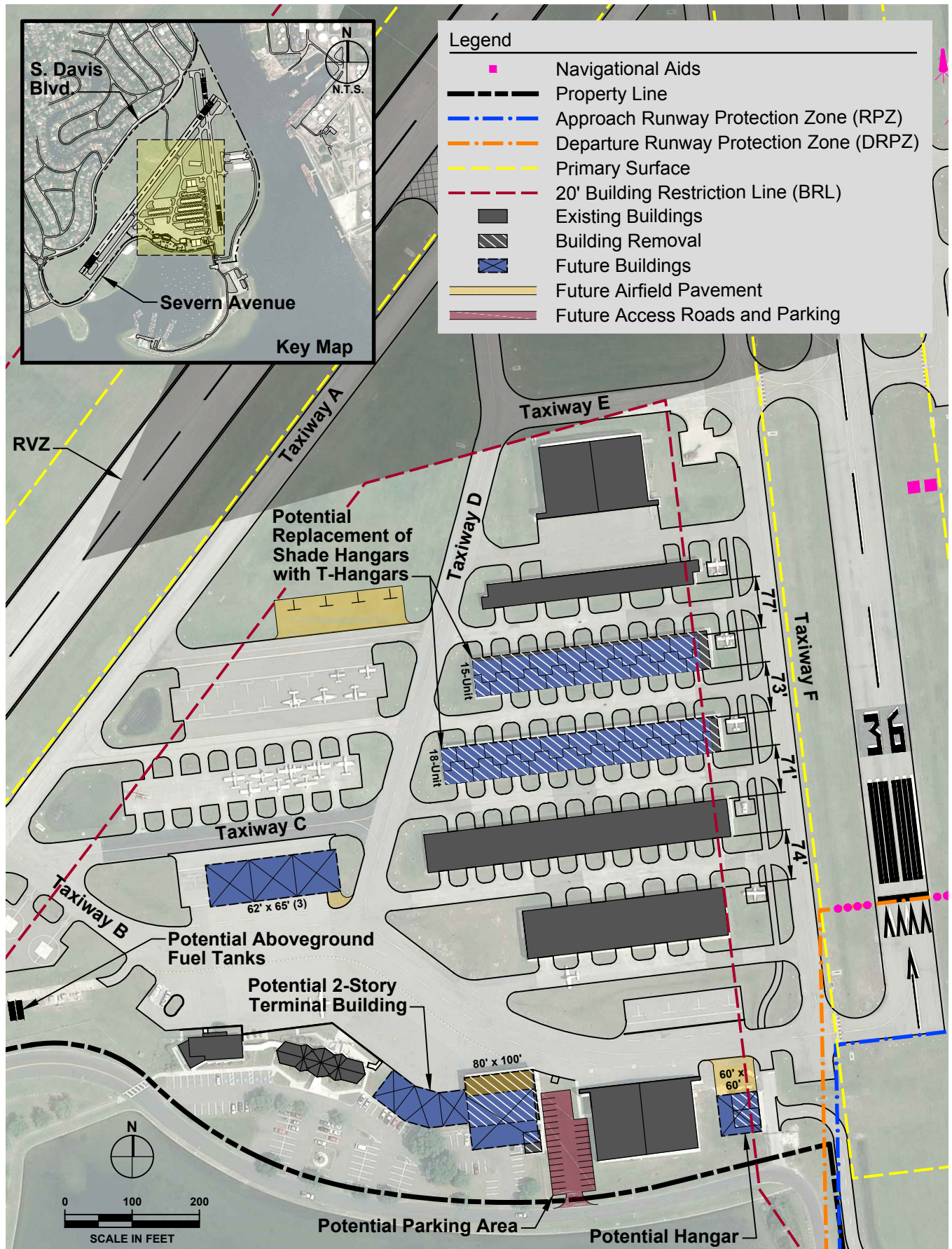
Figure 5-5 Terminal Area Development Alternative
