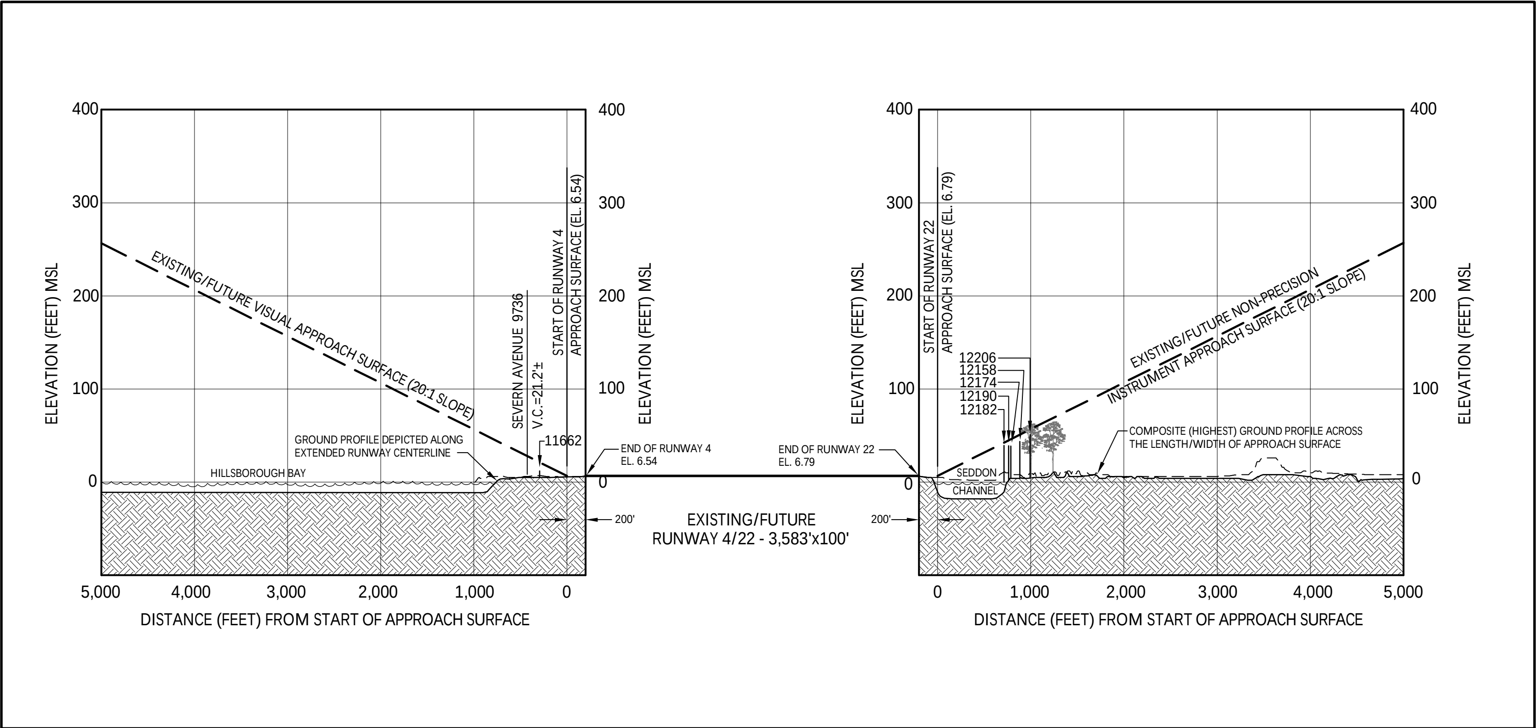
RUNWAY 4/22 PROFILE VIEW
