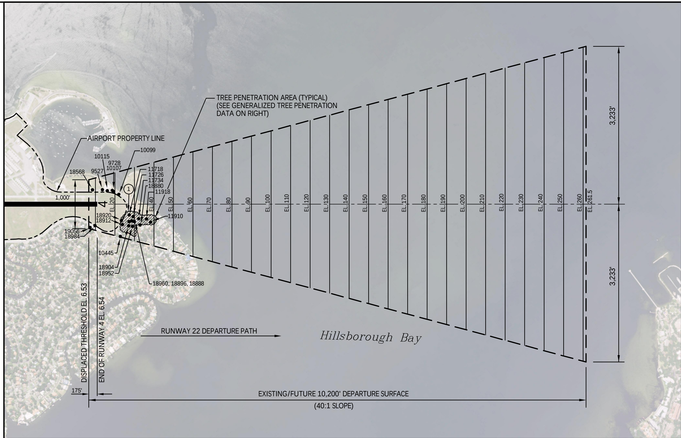
RUNWAY 22 DEPARTURE SURFACE PLAN VIEW
