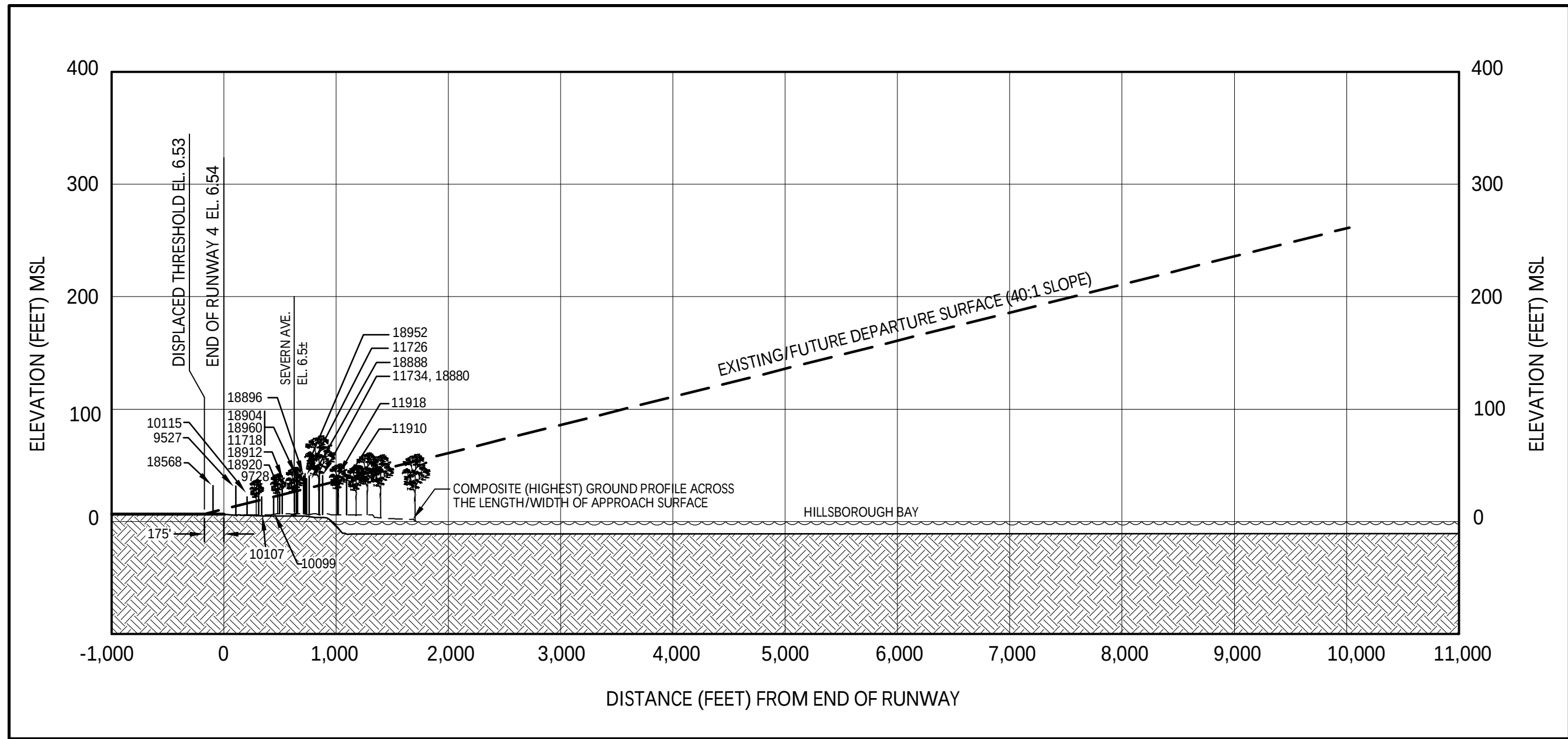
RUNWAY 22 DEPARTURE SURFACE PROFILE VIEW
